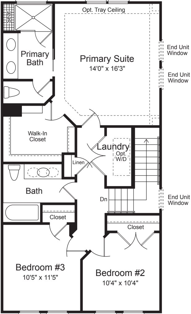
THIRD LEVEL PLAN
