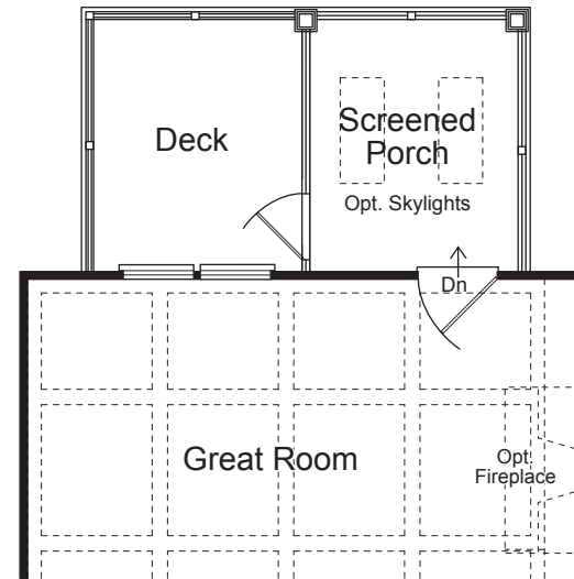
OPT. HALF SCREENED PORCH AND DECK
