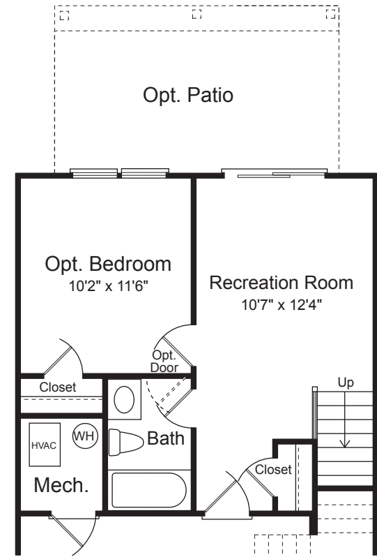
OPT. 1ST. FLOOR BEDROOM/ OPT. 1ST. FLOOR BATH
